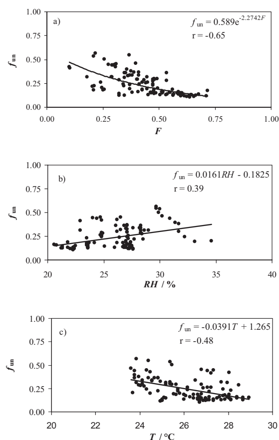
Figure 3. Dependence of f_{\text{un}} – the fraction of unattached short-lived radon decay products – on: a) F – equilibrium factor, b) RH – relative indoor air humidity and c) T – indoor air temperature, for the measurements in the s-MO-S3-01 school during the period January 18–27, 2000.
