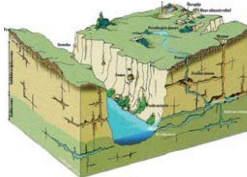
Slika 1: Shematični prikaz krasa (risba R. Kozel). Figure 1: Schematic drawing of the Karst (drawing by R. Kozel).
