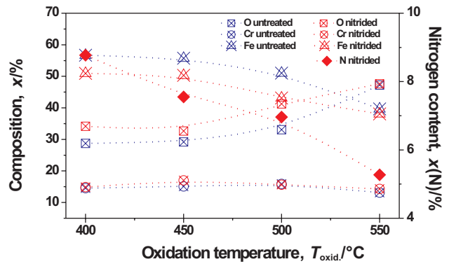
Figure 16: EDS surface composition of the oxidised surfaces of both untreated (blue) and nitrided (red) as a function of the oxidation temperature
