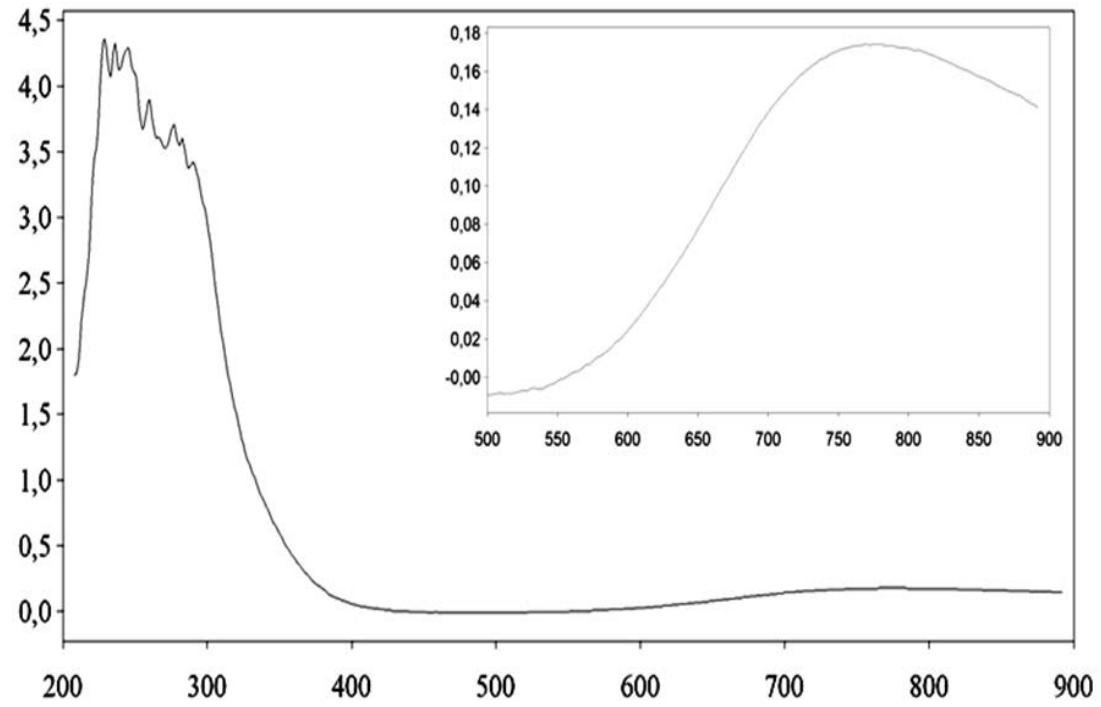
Figure S2. Electronic Spectrum of [\text{Cu}_3(\mu_2\text{-Cl})_2\text{Cl}_4(2\text{-Vim})_6]
