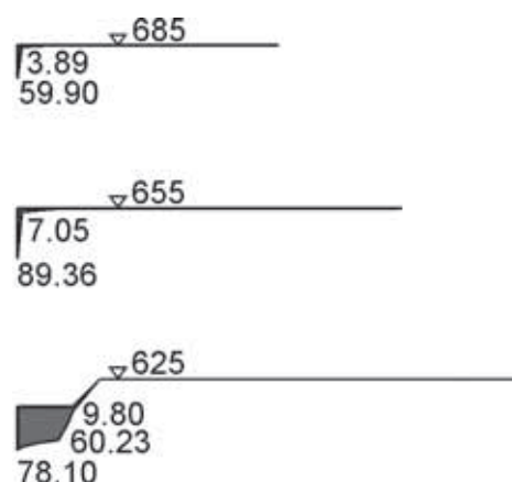
Figure 6. Uplift pressure head contour lines.
