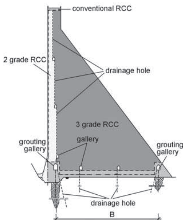
Figure 2. Cross section of seepage control measures for RCCD.
