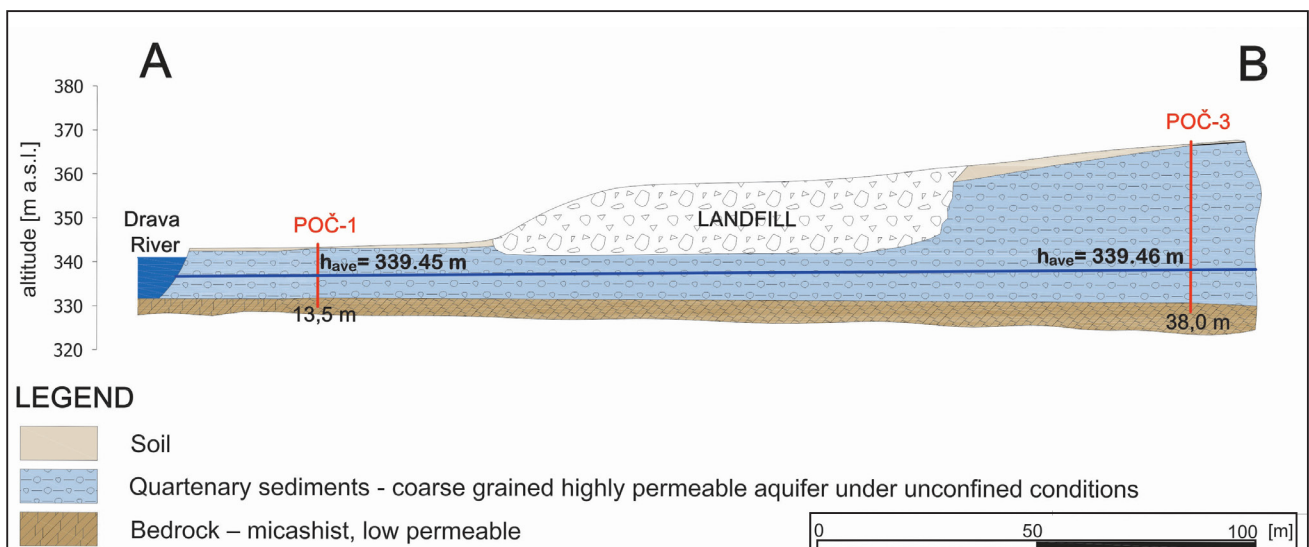
Fig. 2. Hydrogeological profile (for the position see Fig. 1).
