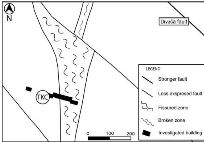
Figure 2. Structural map of the Divača site and position of the TKC room.
