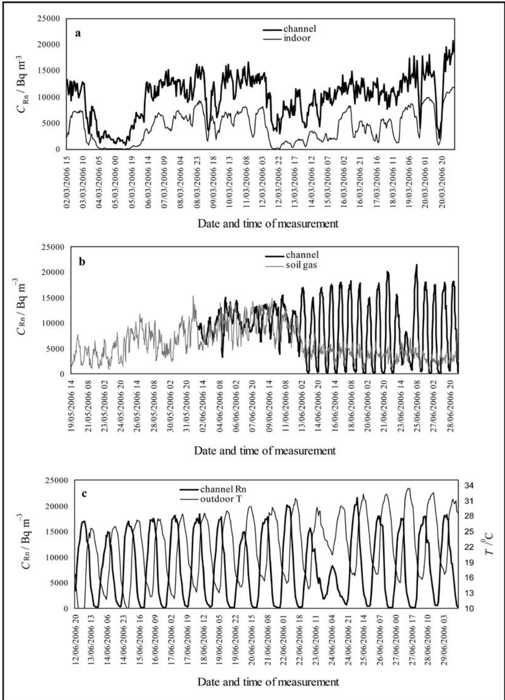
Figure 4. Relationships between a) radon concentration in indoor and channel air, b) radon concentration in the channel air and soil gas, and c) radon concentration in the channel air and outdoor air temperature.
