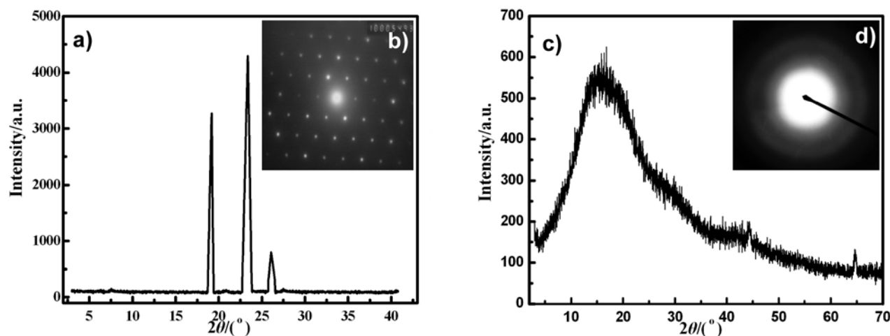
Figure 3. TEM diffraction photographs and XRD pattern for: a), b) PEG1000 homopolymer; c), d) P(MMA-co-VP)/PEG1000 semi-IPNs networks.
