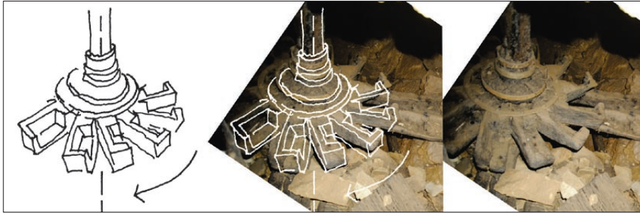
Fig. 10: Wooden waterwheel (turbine): carpentry work, axle, drive spindle and scoops (blades, locally lopaticice pl. ). In Kusalovića mlinica , the security hoops around the scoops ( osiguravajući obruči ) are missing; and the spout of water ( mlaznica ), the base anchor frame ( kobila ) is not visible (Juvanec 2015b).
