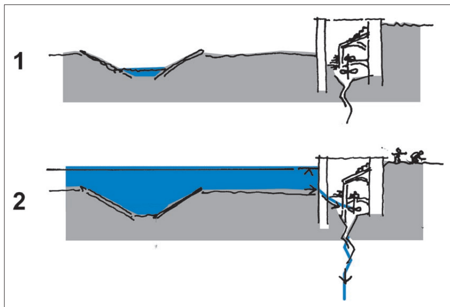
Fig. 7: Water levels of the Trebišnjica river: 1 normal level in the riverbed, practically 100 days in the year; 2 flood level (Juvanec 2015b).
