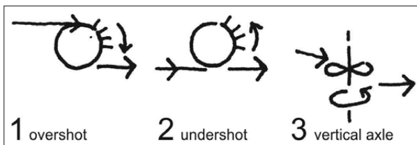
Fig. 2: Drive directions of wheels: overshot (clockwise) and undershot (anticlockwise) principles, and simplification of the Pelton's turbine with vertical axle (Juvanec 2015b).
