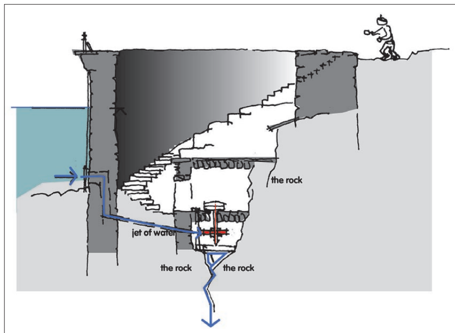
Fig. 9: Documentation: cross section of Kusalovića mlinica at Poljice Popovo. The roof has collapsed and the wooden shutter for the water has been replaced with steel machinery (Juvanec 2015b).
