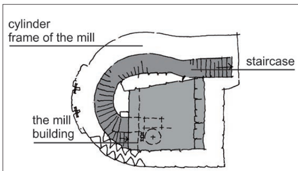
Fig. 11: Ponor mlinica – elements: cylinder or outer walls; mill with three rooms; staircase from the top (terrain). Rectangle in the mill is used as the entrance to the power wheel room, and the circle represents the millstones in the upper room (Juvanec 2015b).
