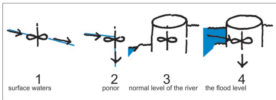
Fig. 4: Theory, the principle of a mill with vertical axle – 1 the stream comes and drains on the surface; 2 the stream comes on the surface and drains into the underground hole; 3 ponor mill and the river at normal level; 4 seasonal use of flood water in Popovo polje (Juvanec 2015b).
