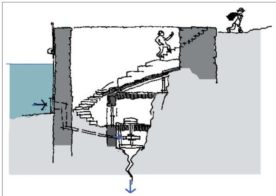
Fig. 12: Reconstruction: cross section with all existing elements and reconstructed roof of stone plates. A steel shutter has replaced original wooden device for opening the spout for the water (Juvanec 2015b).
