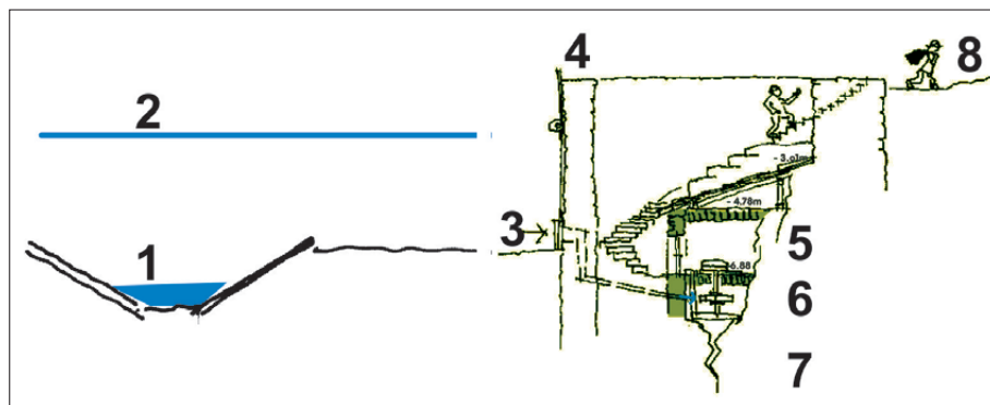
Fig. 8: Elements of the ponor mill: 1 normal level of the water in the riverbed; 2 flood level; 3 entrance of water to the mill; 4 the cylinder, walls around the mill house; 5 miller's room; 6 room with turbine; 7 swallow hole or ponor; 8 entrance from the terrain (Juvanec 2015b).
