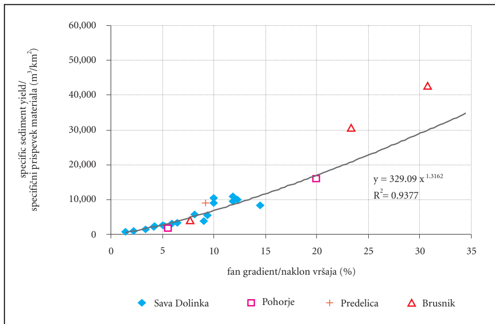
Figure 8: Relation between the specific sediment yield, computed using the Ceriani et al. (2000) method, and the torrential fan gradient for all investigated torrential watersheds (the regression line is Eq. (13)).
