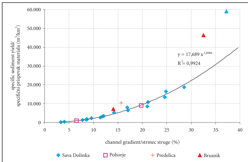
Figure 7: Relation between the specific sediment yield, computed using the method 2 of Marchi & D'Agostino (2002), and the torrential channel gradient for all investigated torrential watersheds (the regression line is Eq. (12)).
