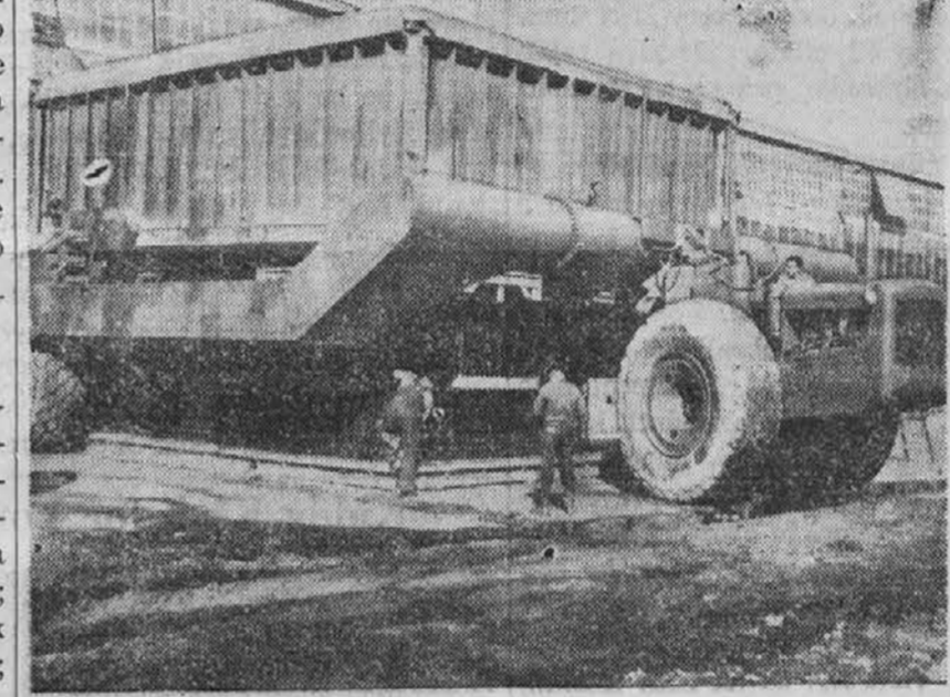
TURN OUT A HOUSE A DAY... New machine developed by R. G. LeTourneau, Peoria, Ill., will turn out a house with two bedrooms in 24 hours. The machine can be rolled into position on a home site on pneumatic tired wheels, pour the concrete and move on to the next site within 24 hours. The mass production idea has been demonstrated to Wilson W. Wyatt, FHA. Unions are expected to object to this type of construction.
